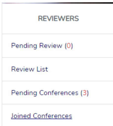
Fig. 4 REVIEWERS menu
